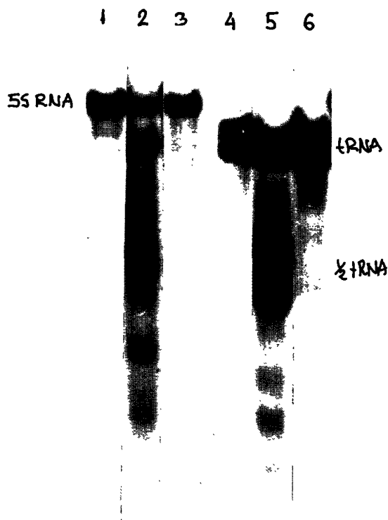
Fig.2. 15% polyacrylamide-7 M urea slab gel electrophoresis of T 1 ribonuclease digest of 32 P-labelled 5 S RNA (slots 1-3) and tRNA (slots 4-6), bound to the preformed tRNA · TP50 complex: (1) initial 5 S RNA; (2) tRNA · TP50 · 5 S RNA*; (3) as (2), but 30 S subunit present; (4) initial tRNA; (5) tRNA · TP50 · tRNA*; (6) as (5), but 30 S subunits present. For details see section 2.
